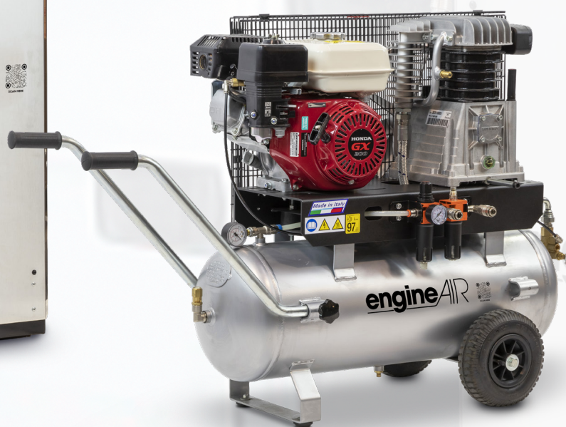
engineAIR 6-50 10 Benzin
