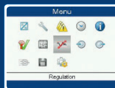
Menu screen
